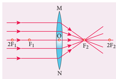
Figure 2.6 Object at infinity
