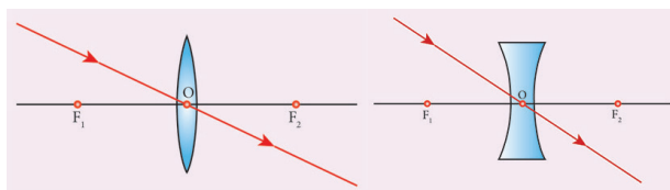
Figure 2.3 Rays passing through the optical centre
