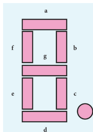
Figure 4.12 Seven segment display
