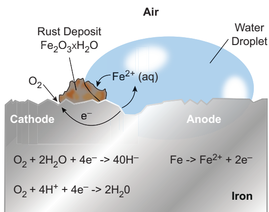
Figure 8.12 Rusting
