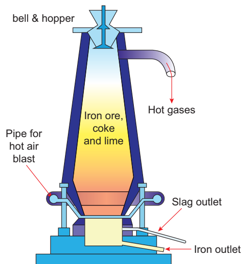
Figure 8.11 Blast Furnace
