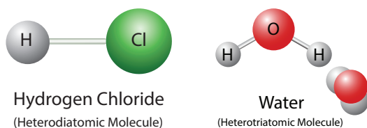
Figure 7.2 Heteroatomic molecules
