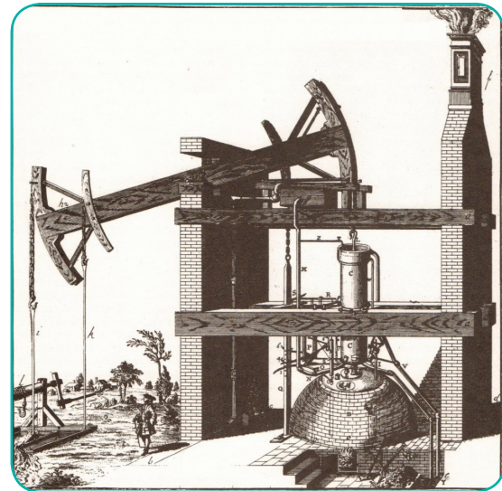
Newcomen Engine lifting coal from mines
