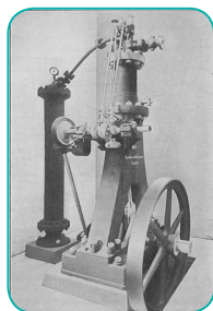
Diesel Engine
