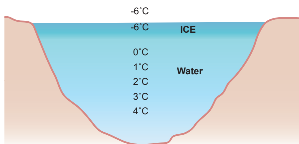
Fig. 10.3 Thermal zones in cold water bodies
