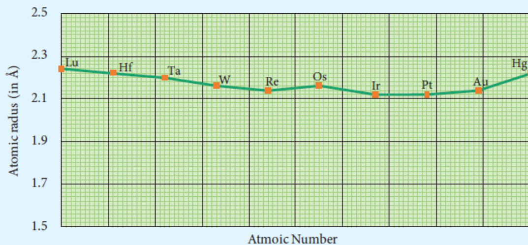
(c) Atomic radius of 5d Elements
