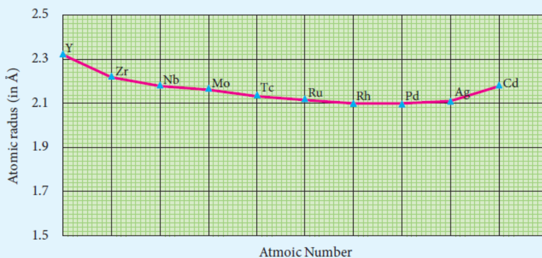
(b) Atomic radius of 4d Elements
