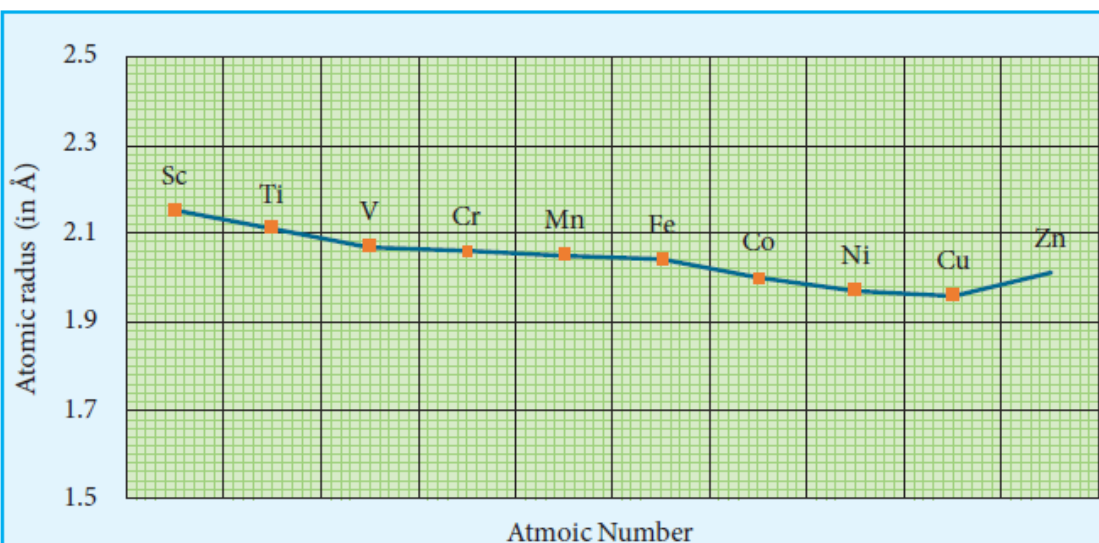
(a) Atomic radius of 3d Elements
